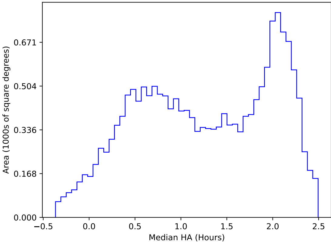
too_elab_r8_d3_gz_v3.4_10yrs WFD y band: Median HA
