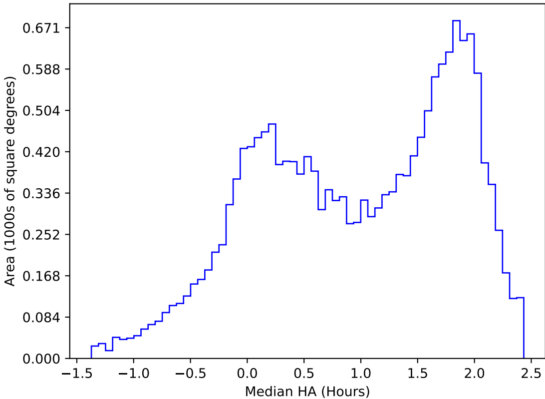
too_elab_r8_d3_gz_v3.4_10yrs WFD u band: Median HA
