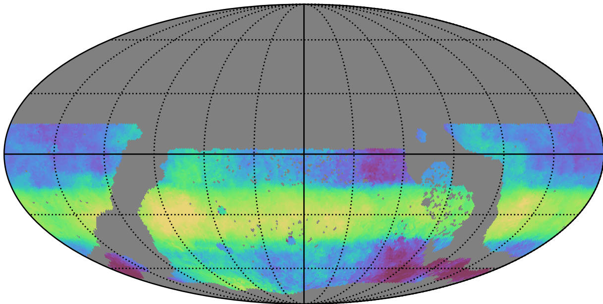
too_elab_r8_d3_gz_v3.4_10yrs WFD r band: Median HA
