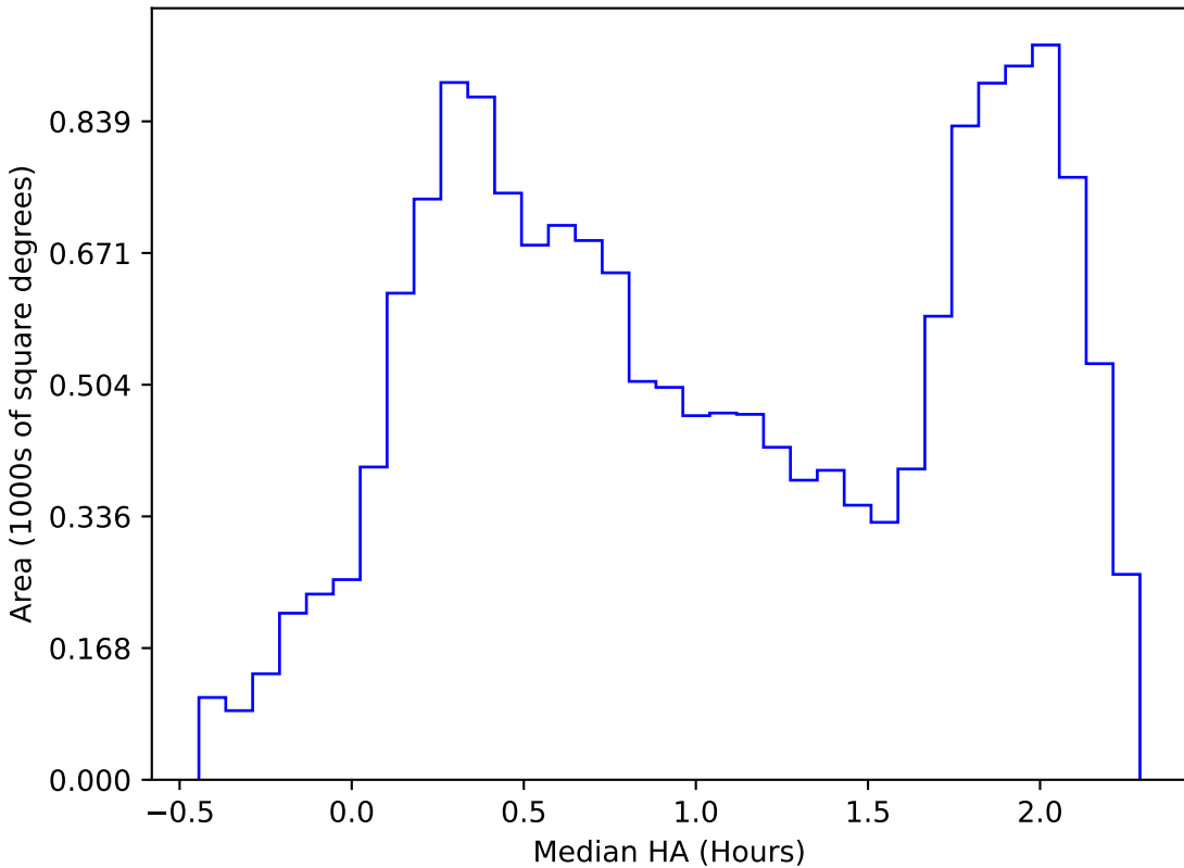
too_elab_r8_d3_gz_v3.4_10yrs WFD i band: Median HA
