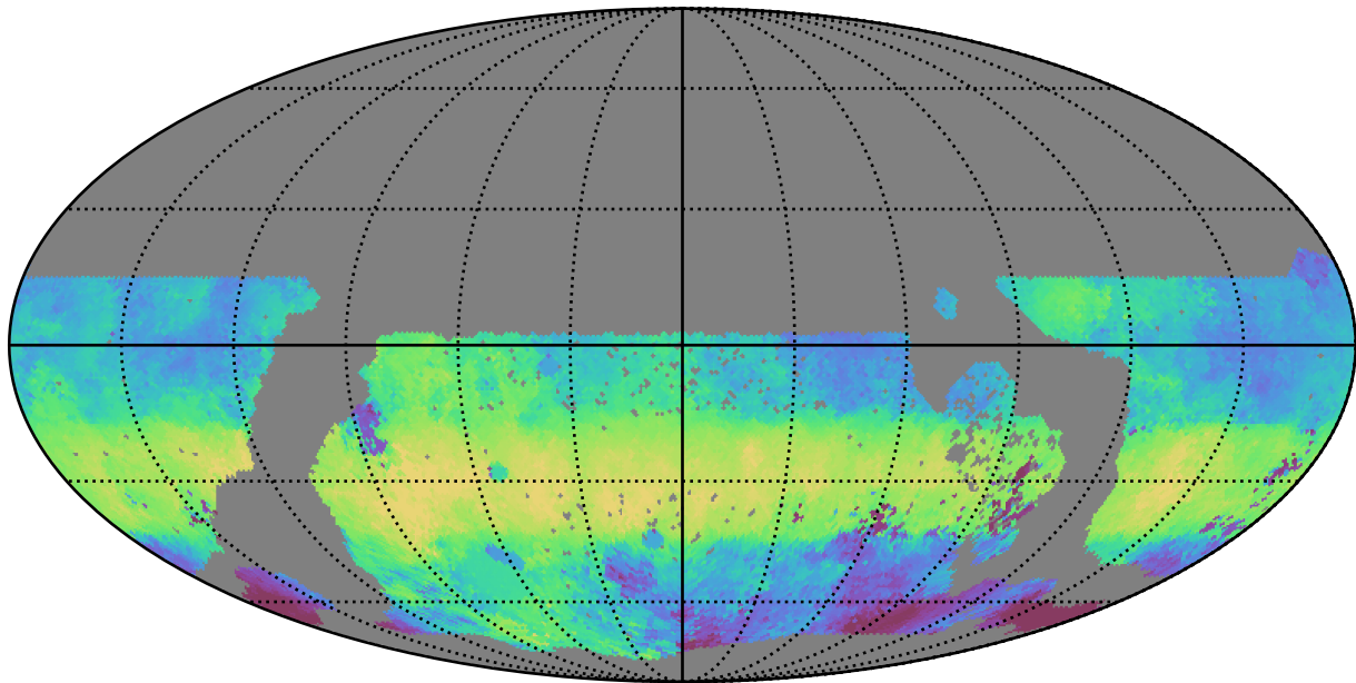
too_elab_r8_d3_gz_v3.4_10yrs WFD g band: Median HA
