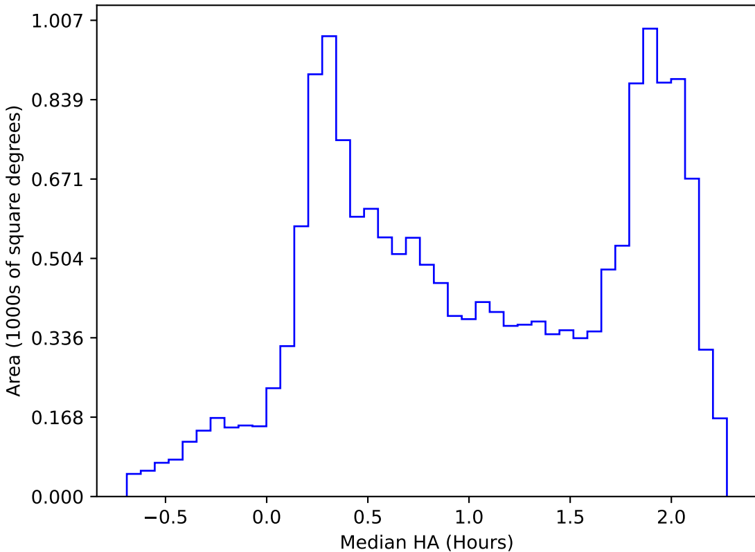
too_elab_r8_d3_gz_v3.4_10yrs WFD all bands: Median HA
