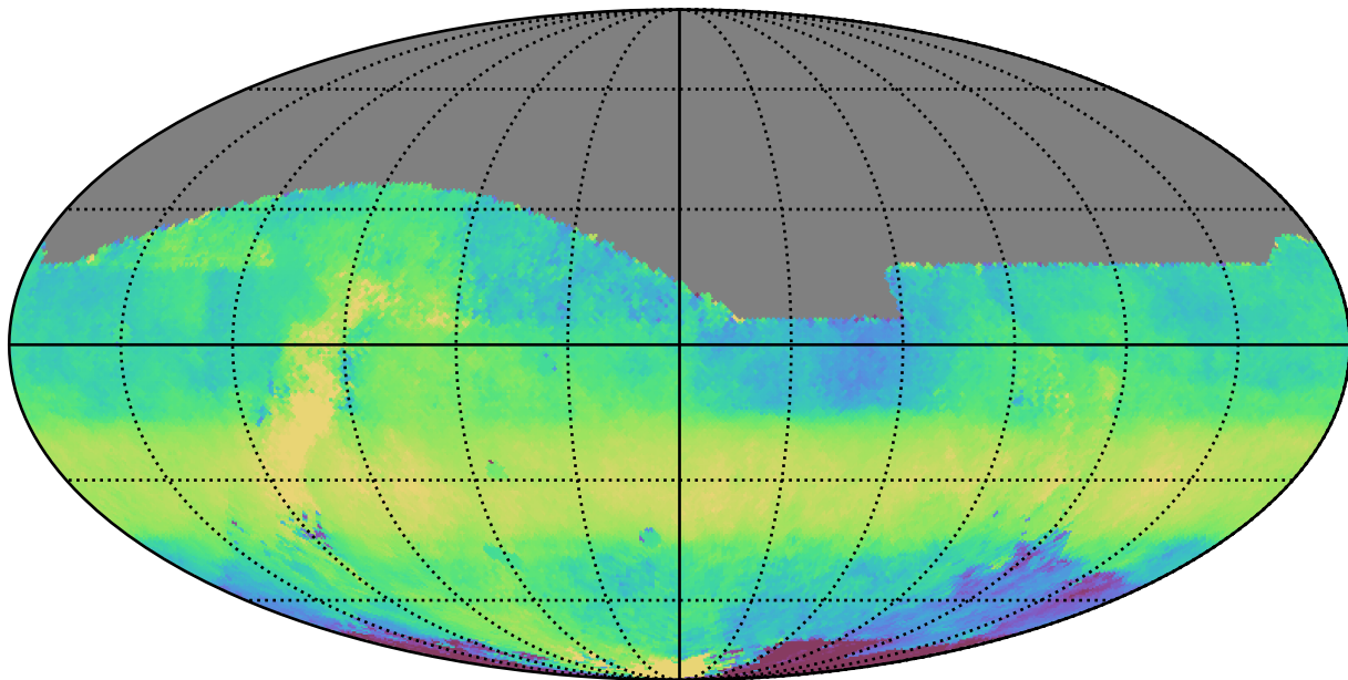
too_elab_r8_d3_gz_v3.4_10yrs All sky z band: Median HA
