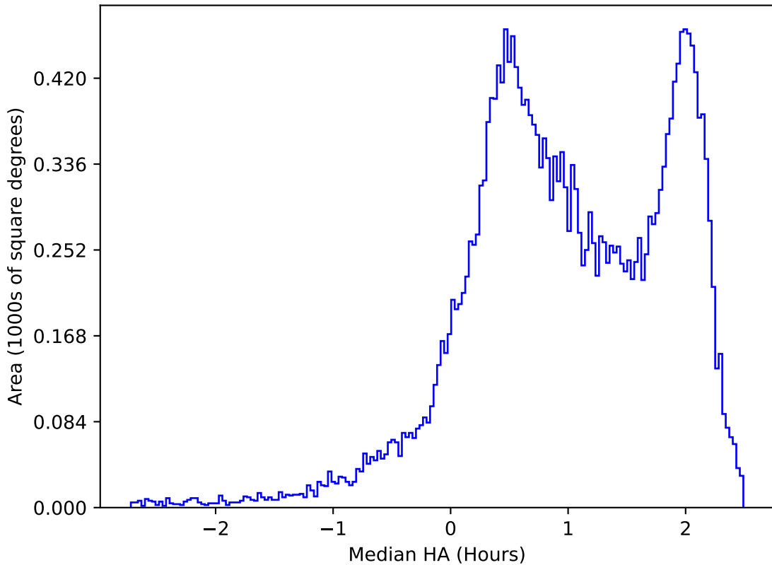
too_elab_r8_d3_gz_v3.4_10yrs All sky z band: Median HA
