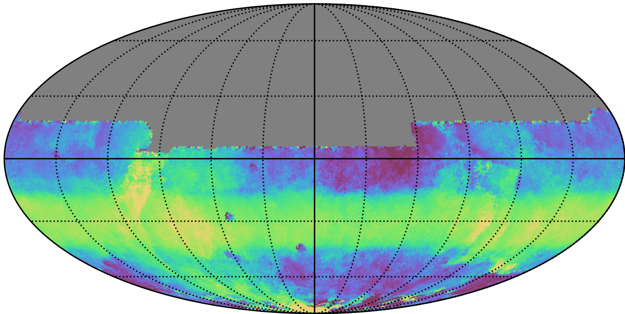
too_elab_r8_d3_gz_v3.4_10yrs All sky y band: Median HA
