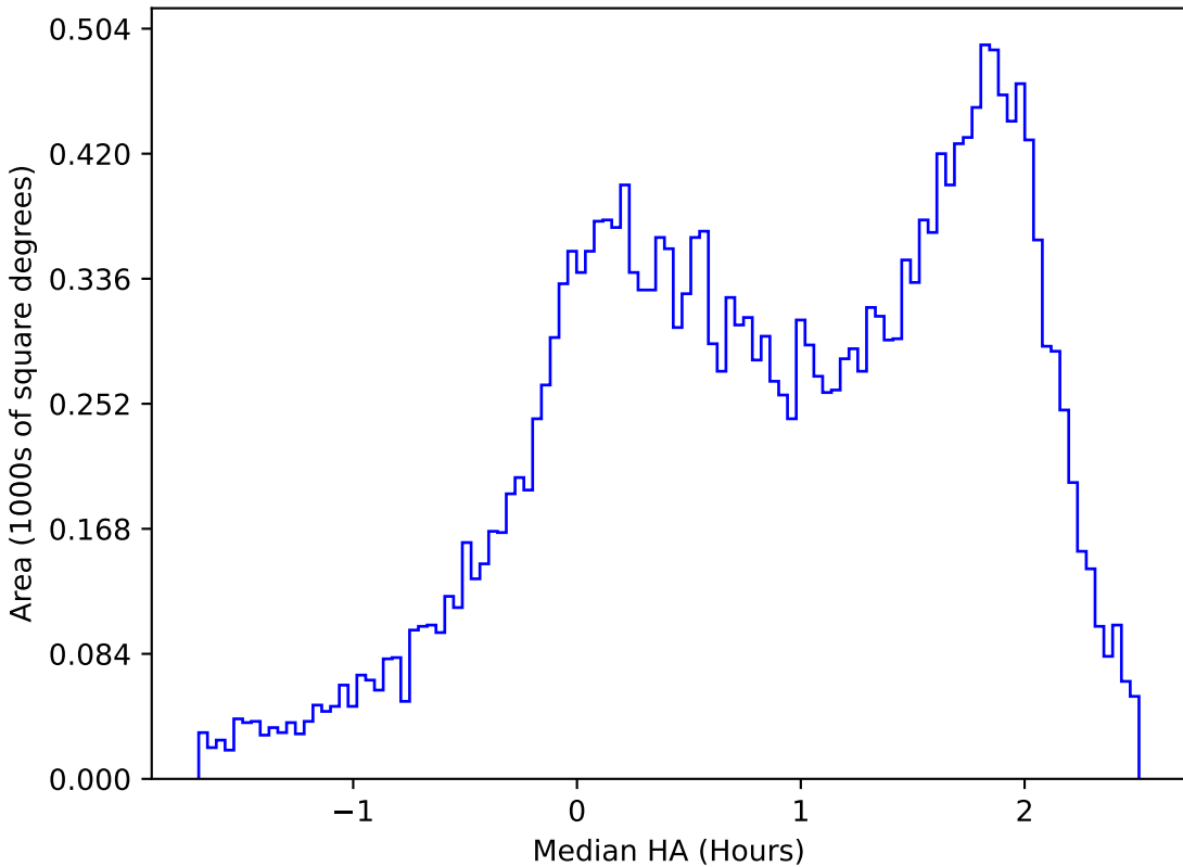
too_elab_r8_d3_gz_v3.4_10yrs All sky u band: Median HA
