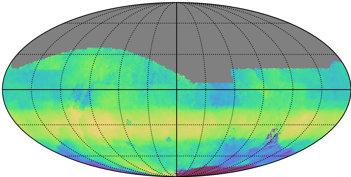
too_elab_r8_d3_gz_v3.4_10yrs All sky r band: Median HA
