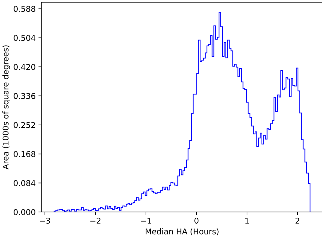
too_elab_r8_d3_gz_v3.4_10yrs All sky r band: Median HA
