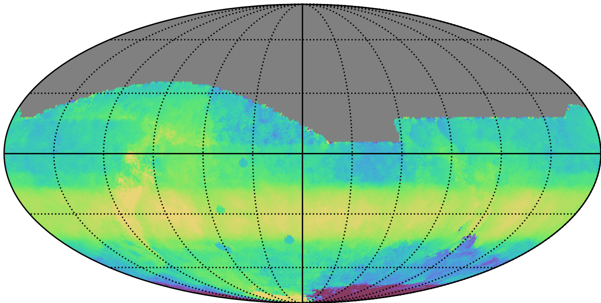
too_elab_r8_d3_gz_v3.4_10yrs All sky i band: Median HA
