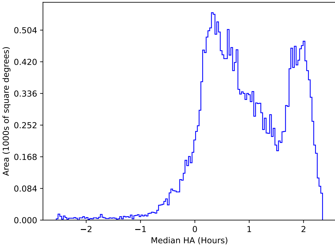
too_elab_r8_d3_gz_v3.4_10yrs All sky i band: Median HA
