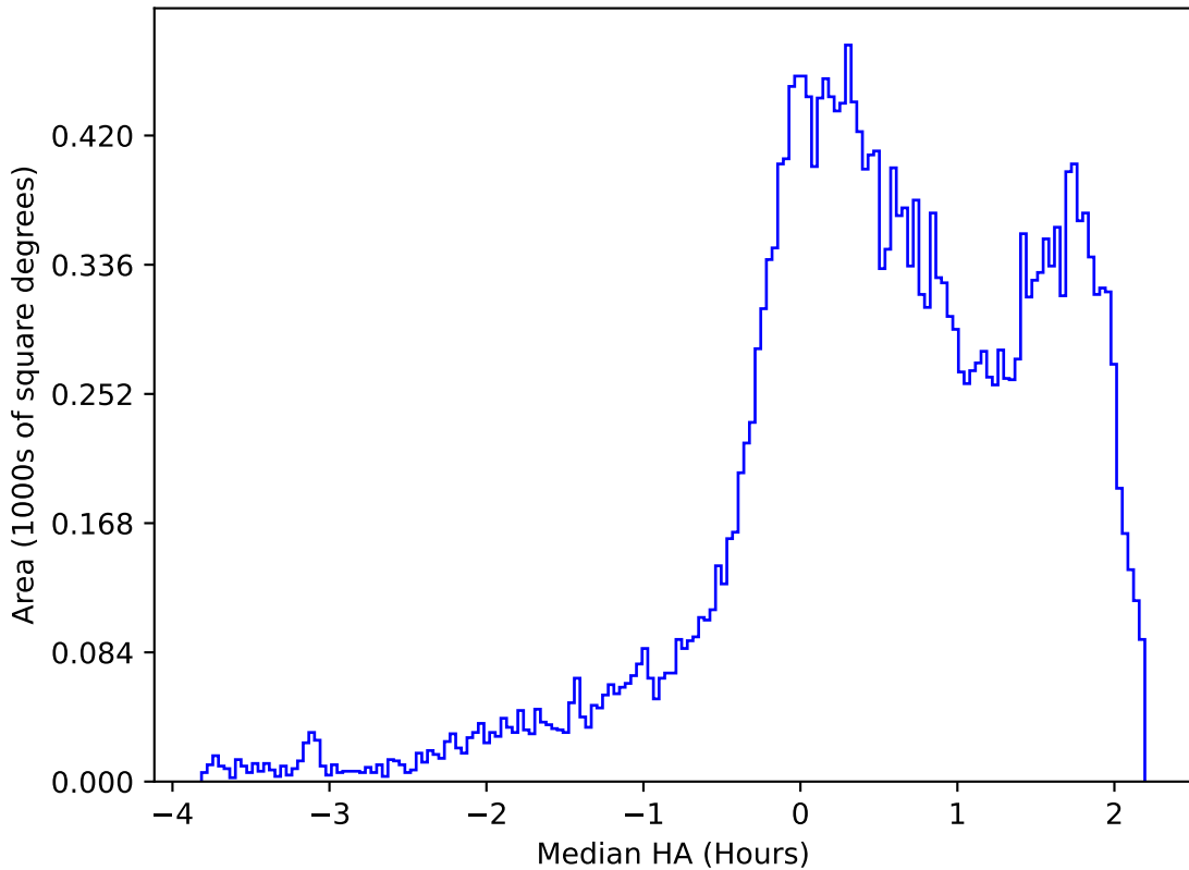
too_elab_r8_d3_gz_v3.4_10yrs All sky g band: Median HA
