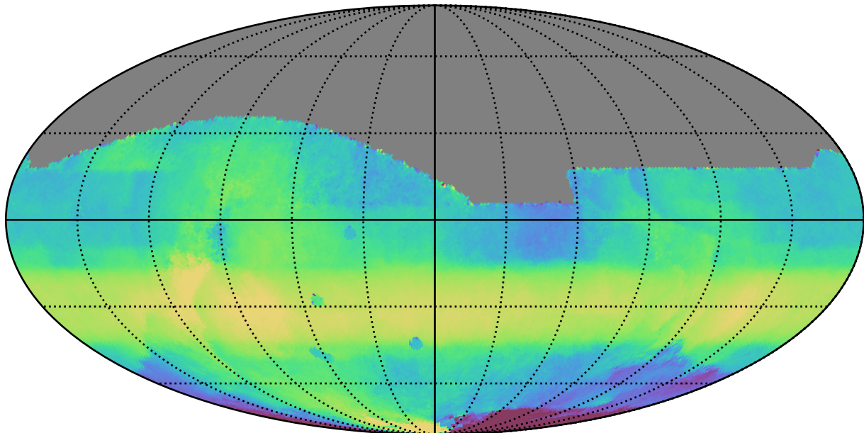
too_elab_r8_d3_gz_v3.4_10yrs All sky all bands: Median HA
