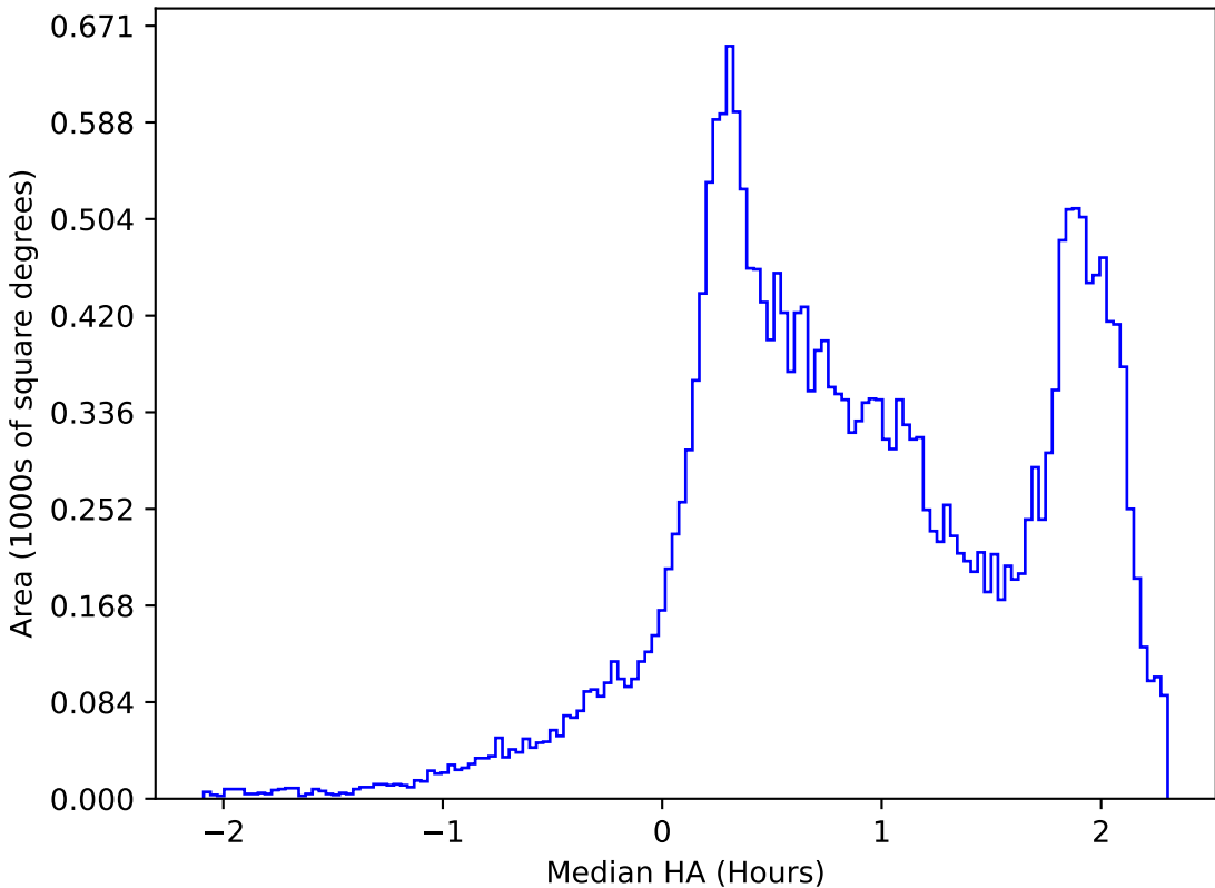
too_elab_r8_d3_gz_v3.4_10yrs All sky all bands: Median HA
