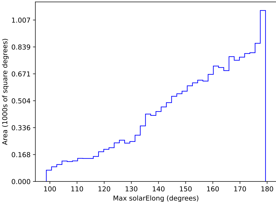
too_elab_r8_d3_gz_v3.4_10yrs WFD z band: Max solarElong
