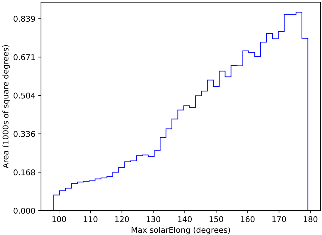
too_elab_r8_d3_gz_v3.4_10yrs WFD g band: Max solarElong
