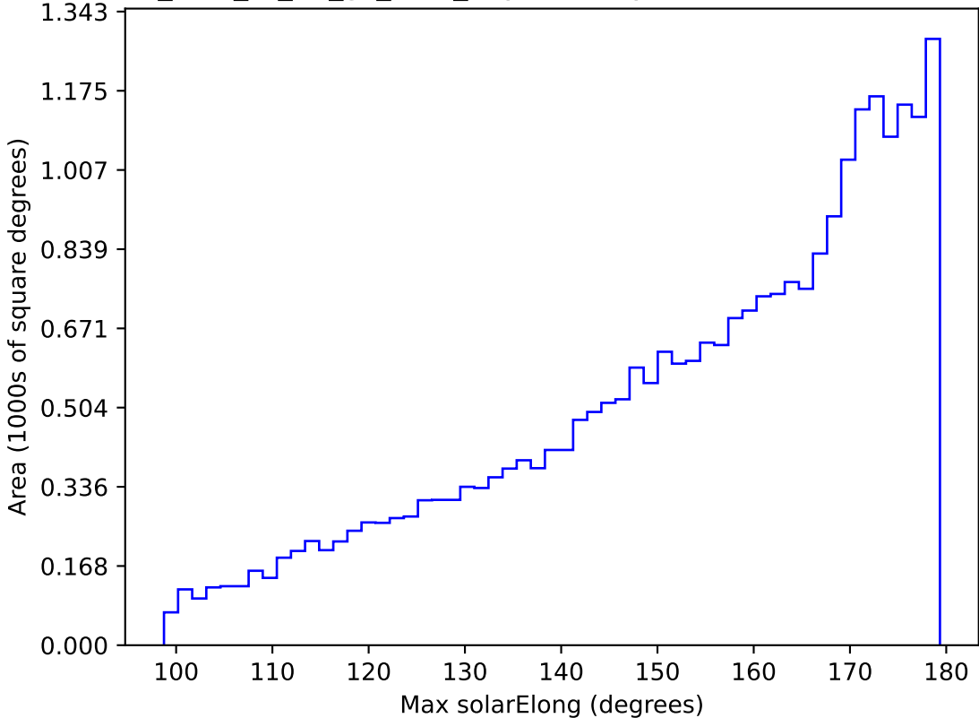
too_elab_r8_d3_gz_v3.4_10yrs All sky z band: Max solarElong
