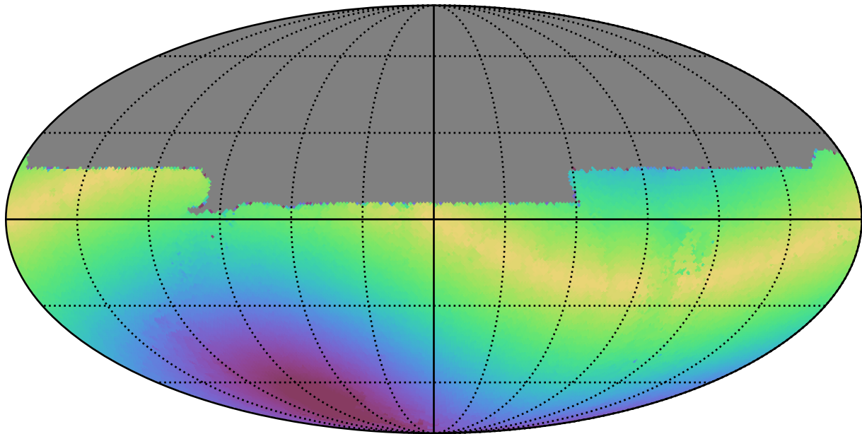
too_elab_r8_d3_gz_v3.4_10yrs All sky u band: Max solarElong
