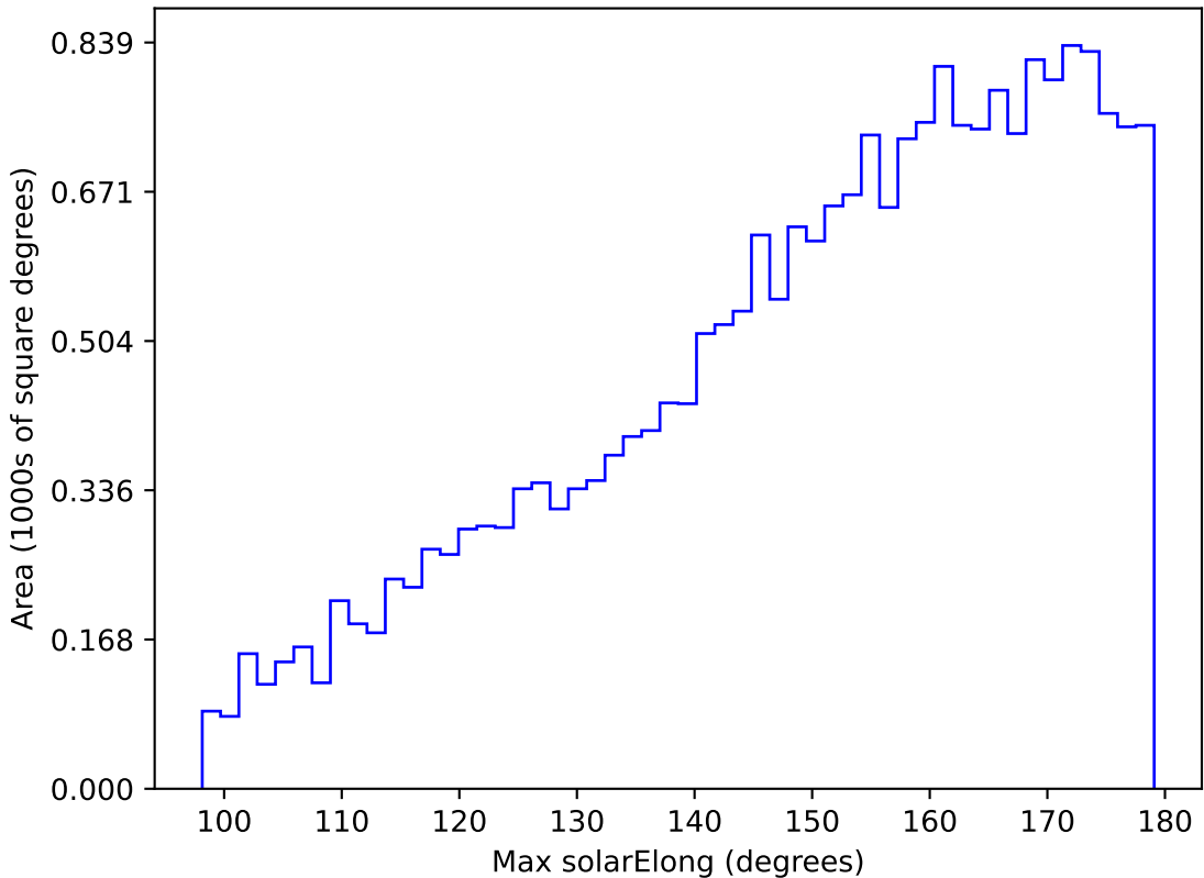
too_elab_r8_d3_gz_v3.4_10yrs All sky u band: Max solarElong
