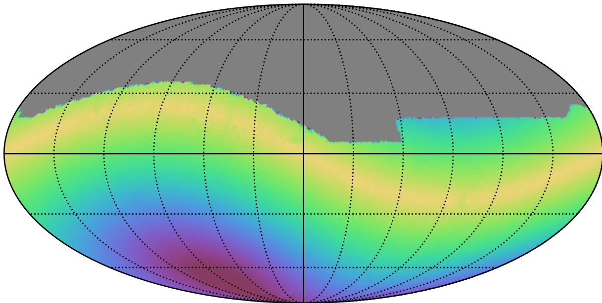
too_elab_r8_d3_gz_v3.4_10yrs All sky i band: Max solarElong
