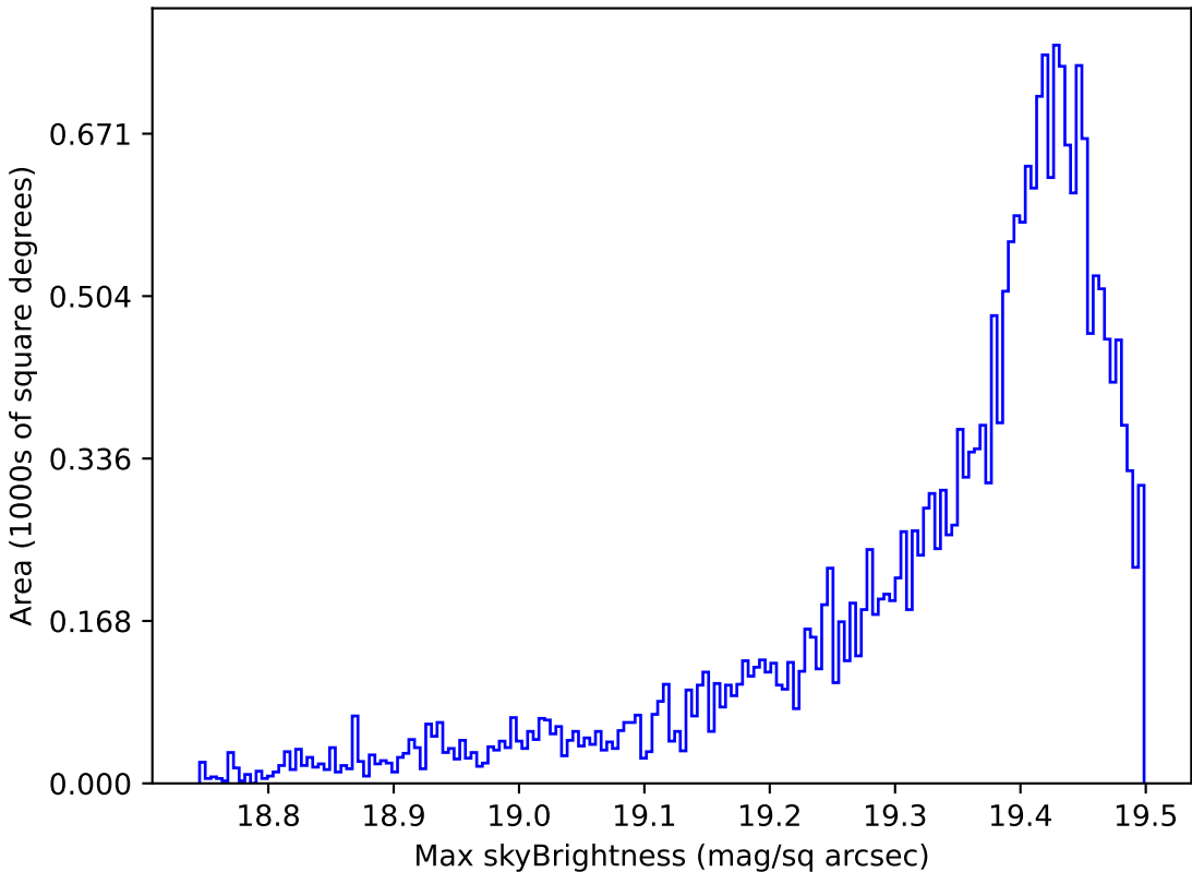
too_elab_r8_d3_gz_v3.4_10yrs Yr 1 z band: Max skyBrightness
