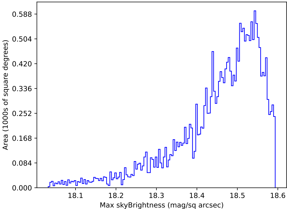
too_elab_r8_d3_gz_v3.4_10yrs Yr 1 y band: Max skyBrightness
