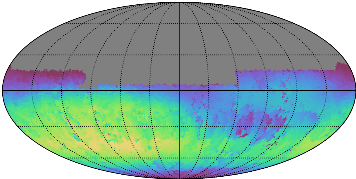
too_elab_r8_d3_gz_v3.4_10yrs Yr 1 u band: Max skyBrightness
