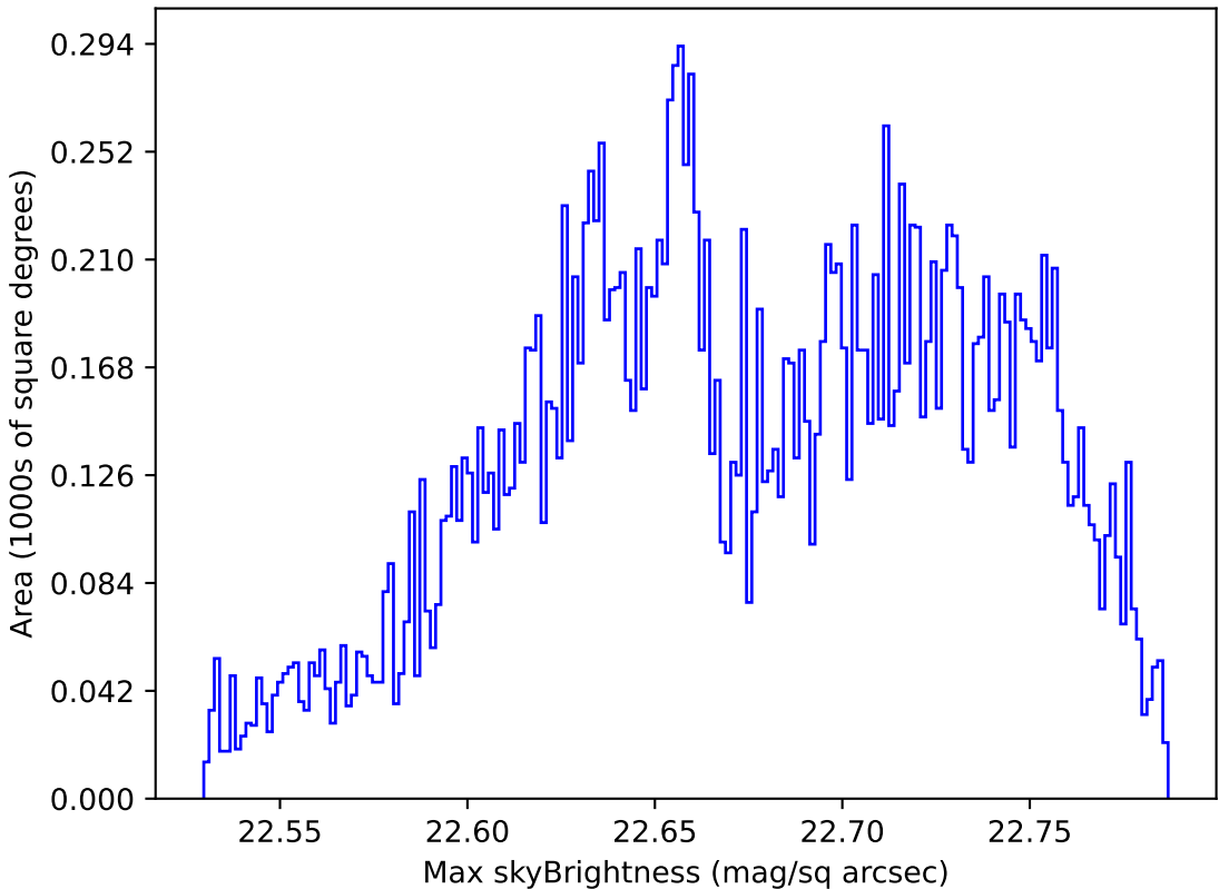
too_elab_r8_d3_gz_v3.4_10yrs Yr 1 u band: Max skyBrightness
