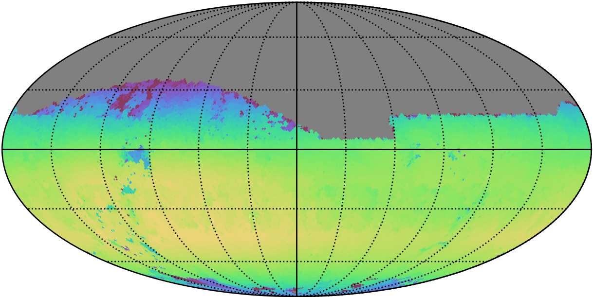
too_elab_r8_d3_gz_v3.4_10yrs Yr 1 i band: Max skyBrightness
