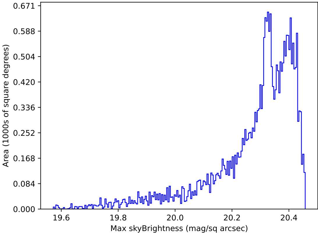
too_elab_r8_d3_gz_v3.4_10yrs Yr 1 i band: Max skyBrightness
