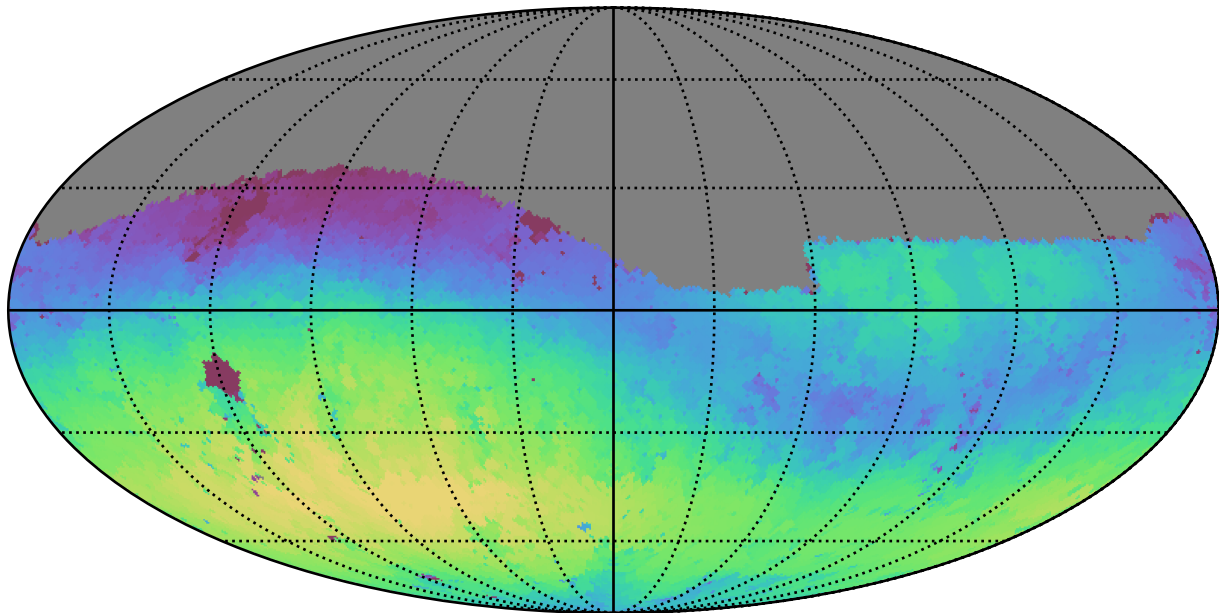
too_elab_r8_d3_gz_v3.4_10yrs Yr 1 g band: Max skyBrightness
