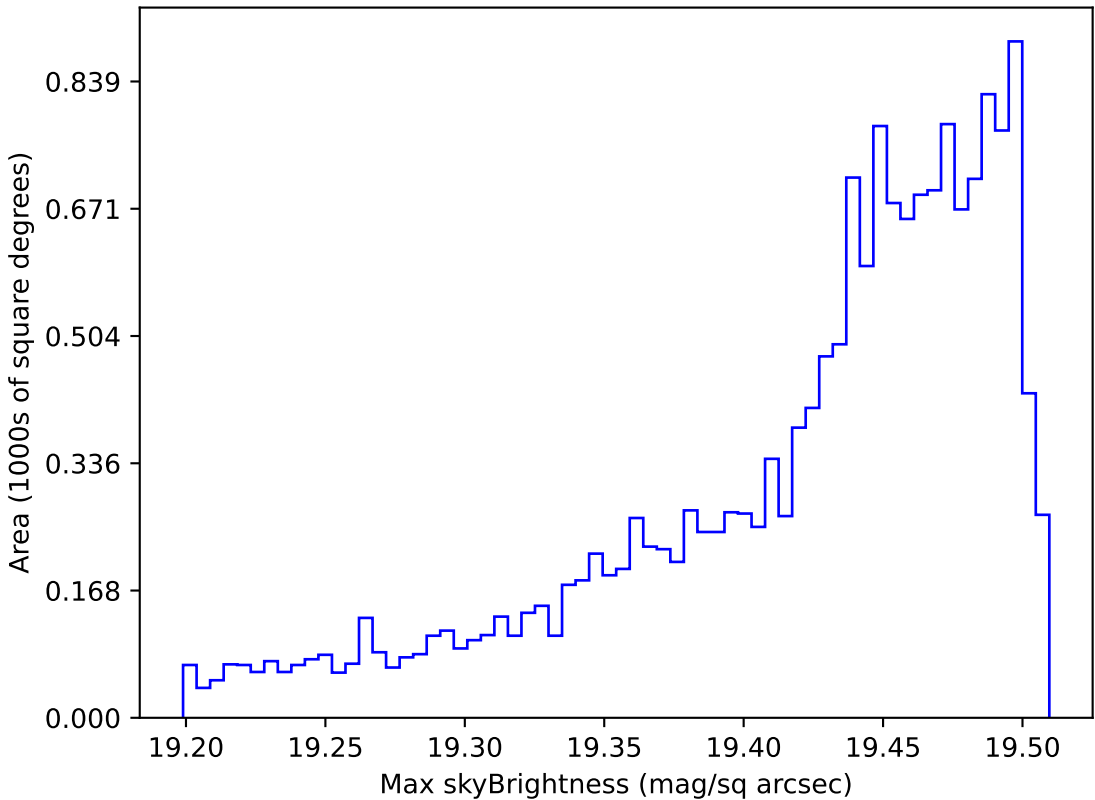
too_elab_r8_d3_gz_v3.4_10yrs WFD z band: Max skyBrightness
