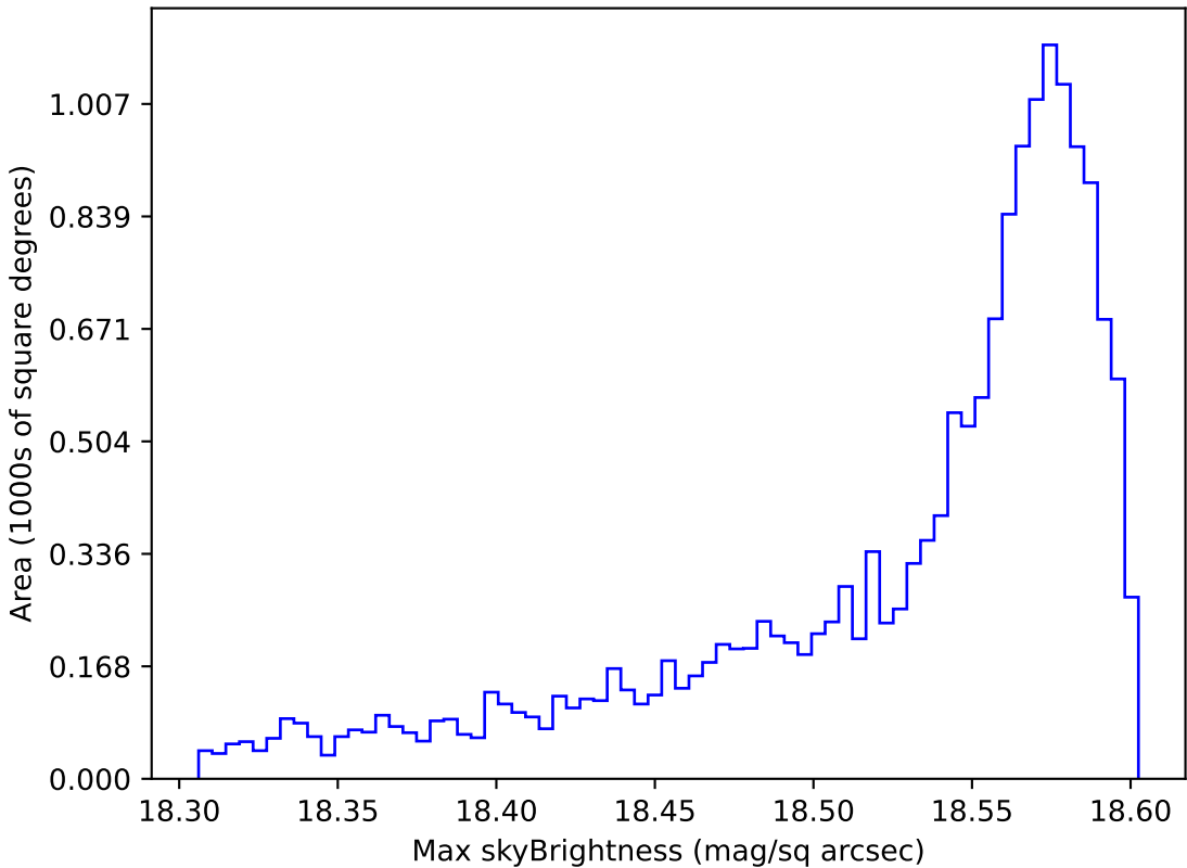
too_elab_r8_d3_gz_v3.4_10yrs WFD y band: Max skyBrightness
