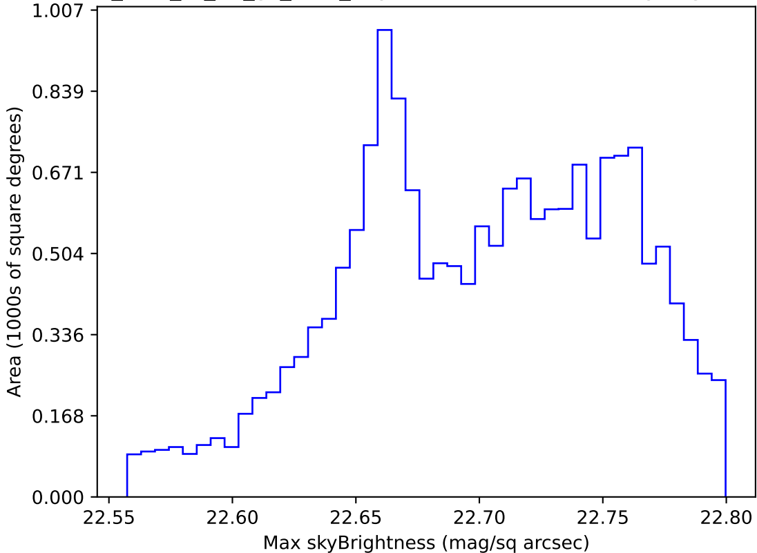
too_elab_r8_d3_gz_v3.4_10yrs WFD u band: Max skyBrightness
