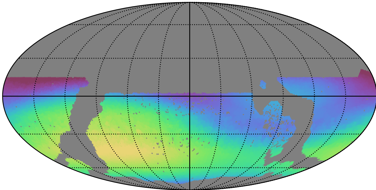
too_elab_r8_d3_gz_v3.4_10yrs WFD r band: Max skyBrightness
