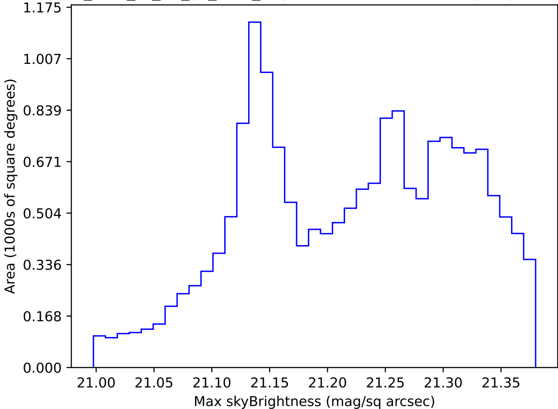
too_elab_r8_d3_gz_v3.4_10yrs WFD r band: Max skyBrightness
