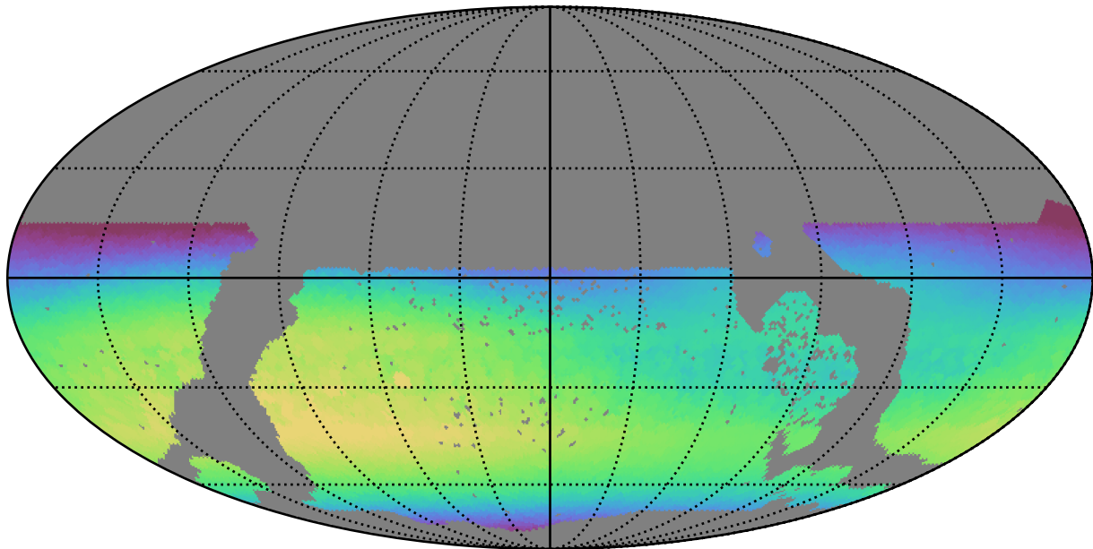
too_elab_r8_d3_gz_v3.4_10yrs WFD i band: Max skyBrightness
