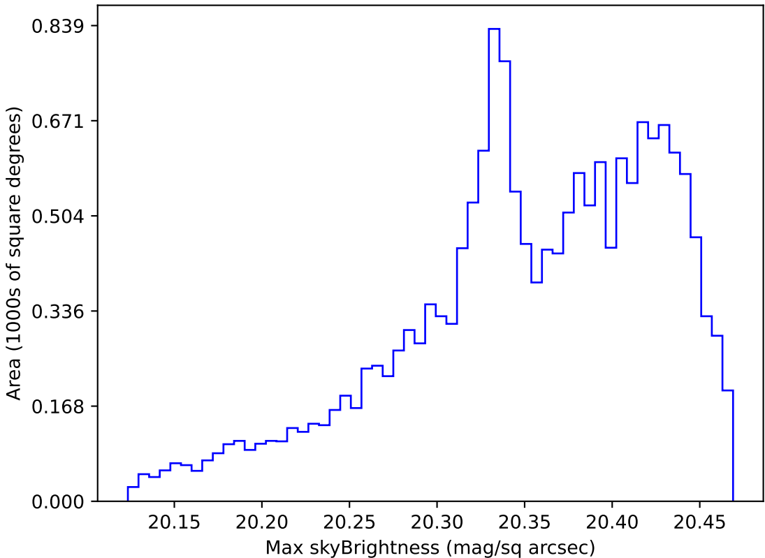
too_elab_r8_d3_gz_v3.4_10yrs WFD i band: Max skyBrightness
