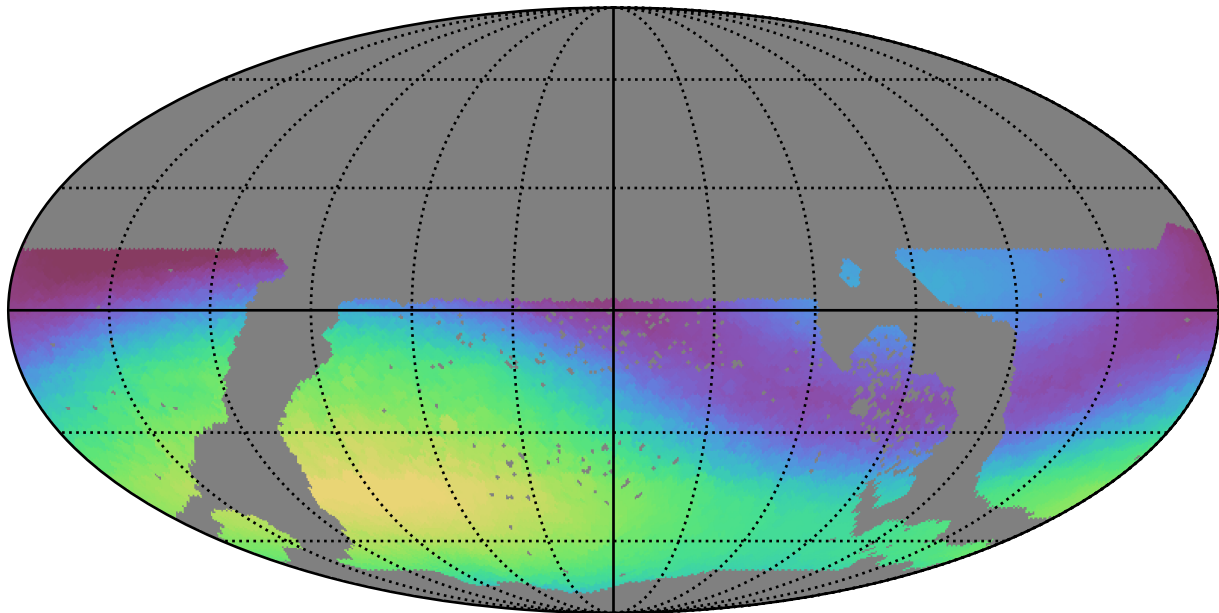
too_elab_r8_d3_gz_v3.4_10yrs WFD g band: Max skyBrightness
