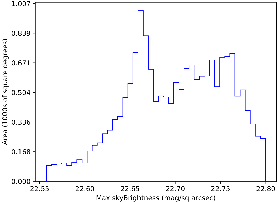
too_elab_r8_d3_gz_v3.4_10yrs WFD all bands: Max skyBrightness
