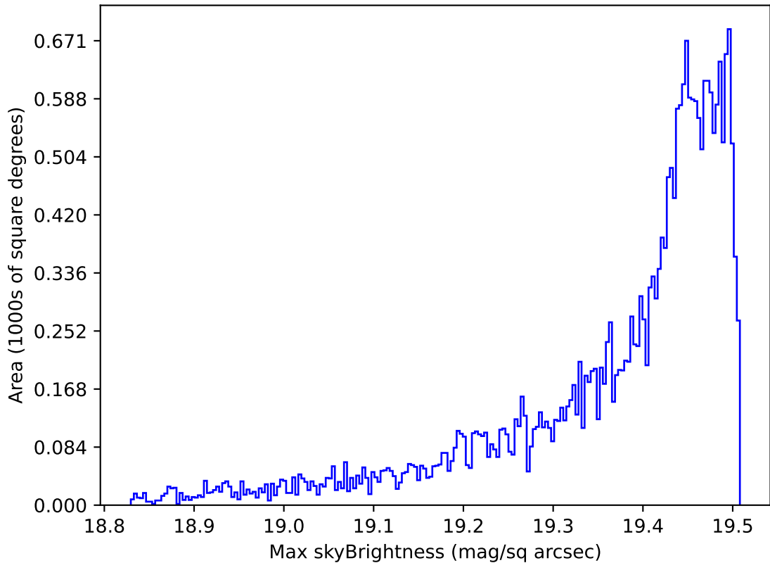
too_elab_r8_d3_gz_v3.4_10yrs All sky z band: Max skyBrightness
