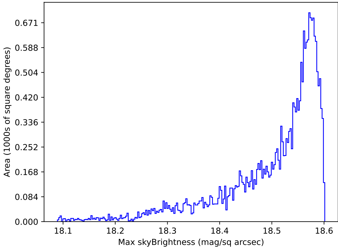
too_elab_r8_d3_gz_v3.4_10yrs All sky y band: Max skyBrightness
