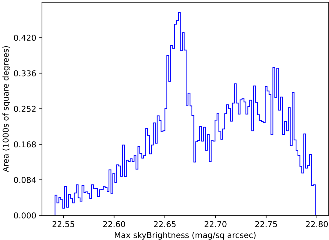
too_elab_r8_d3_gz_v3.4_10yrs All sky u band: Max skyBrightness
