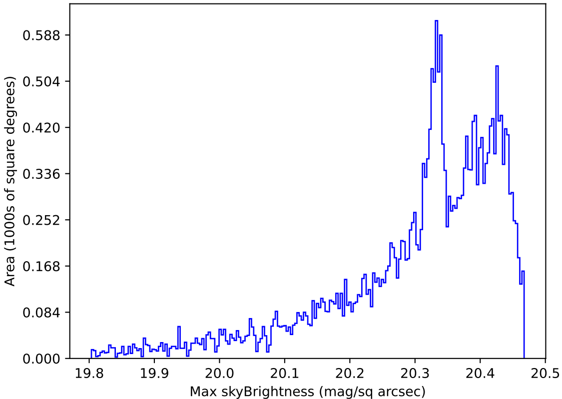
too_elab_r8_d3_gz_v3.4_10yrs All sky i band: Max skyBrightness
