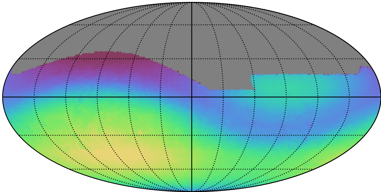
too_elab_r8_d3_gz_v3.4_10yrs All sky g band: Max skyBrightness
