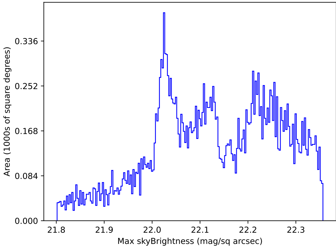
too_elab_r8_d3_gz_v3.4_10yrs All sky g band: Max skyBrightness
