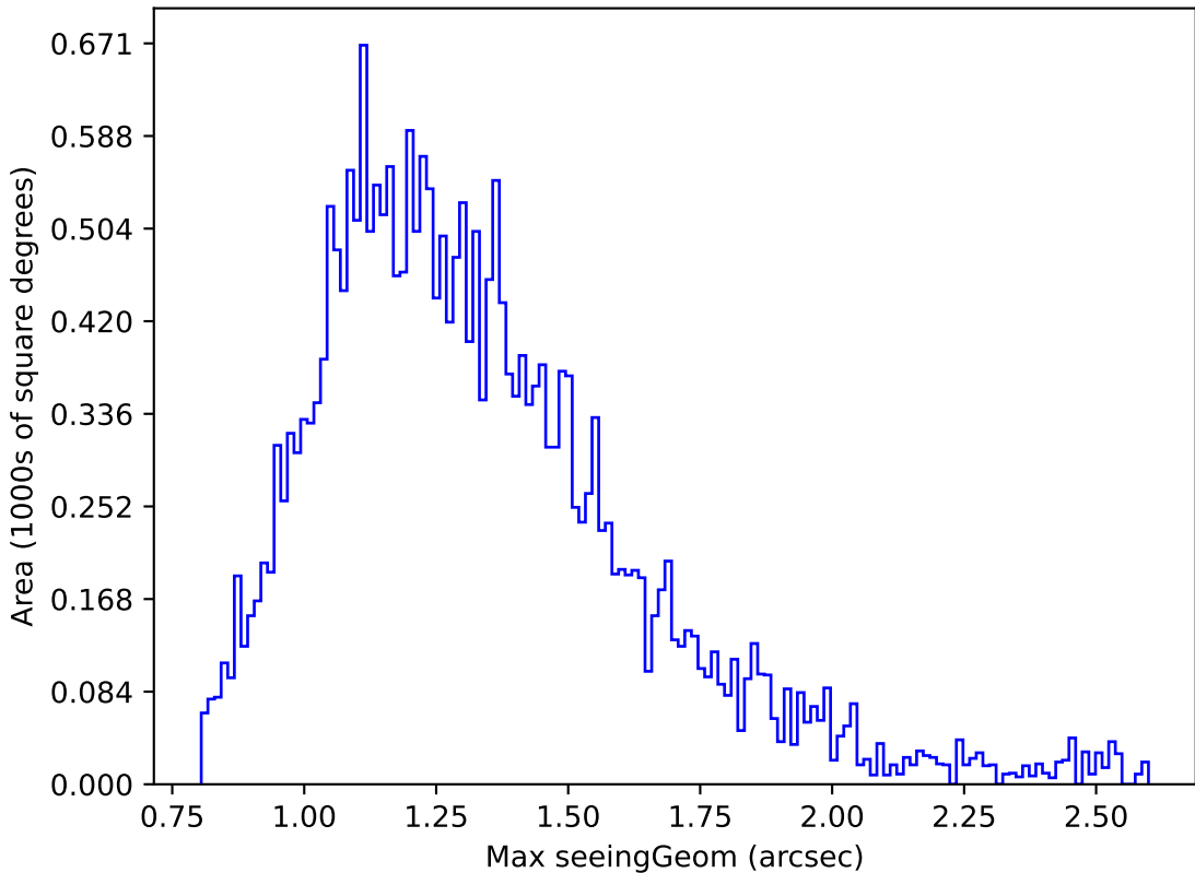
too_elab_r8_d3_gz_v3.4_10yrs Yr 1 z band: Max seeingGeom
