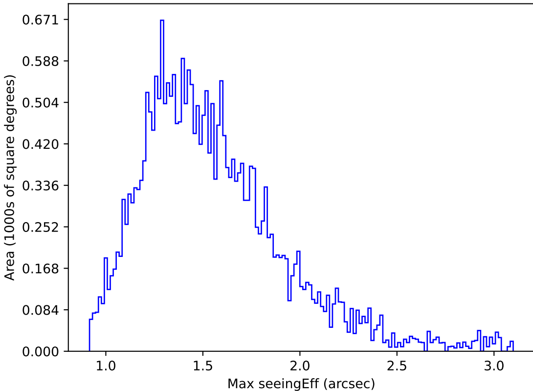
too_elab_r8_d3_gz_v3.4_10yrs Yr 1 z band: Max seeingEff
