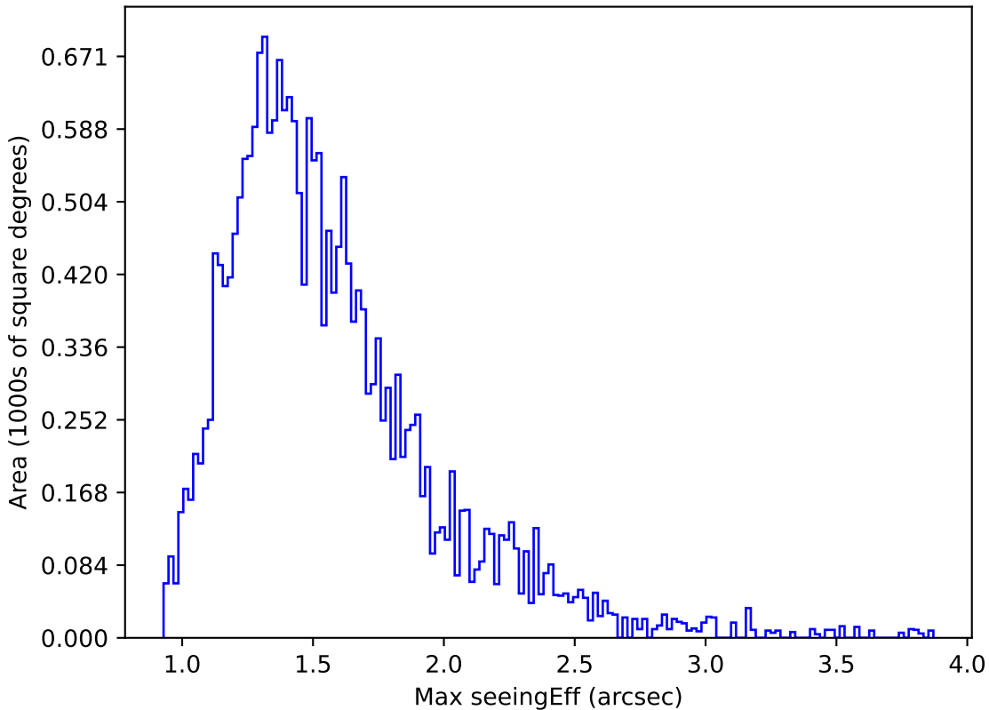
too_elab_r8_d3_gz_v3.4_10yrs Yr 1 u band: Max seeingEff
