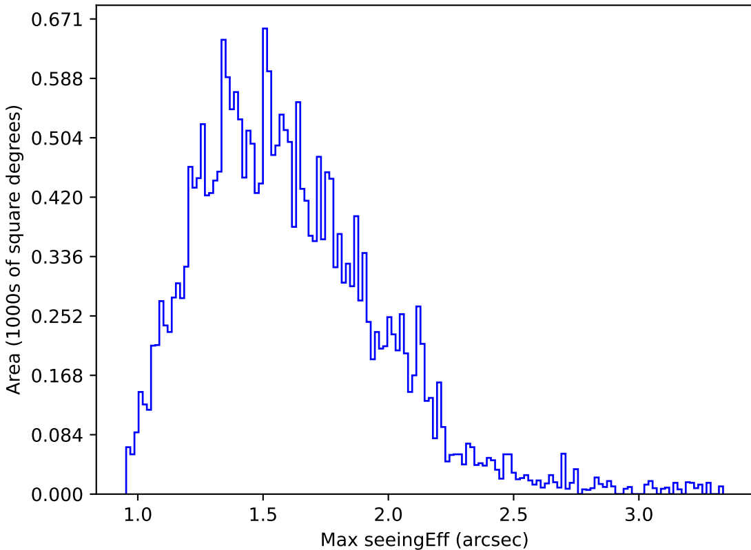
too_elab_r8_d3_gz_v3.4_10yrs Yr 1 r band: Max seeingEff
