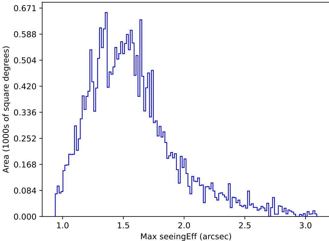
too_elab_r8_d3_gz_v3.4_10yrs Yr 1 g band: Max seeingEff
